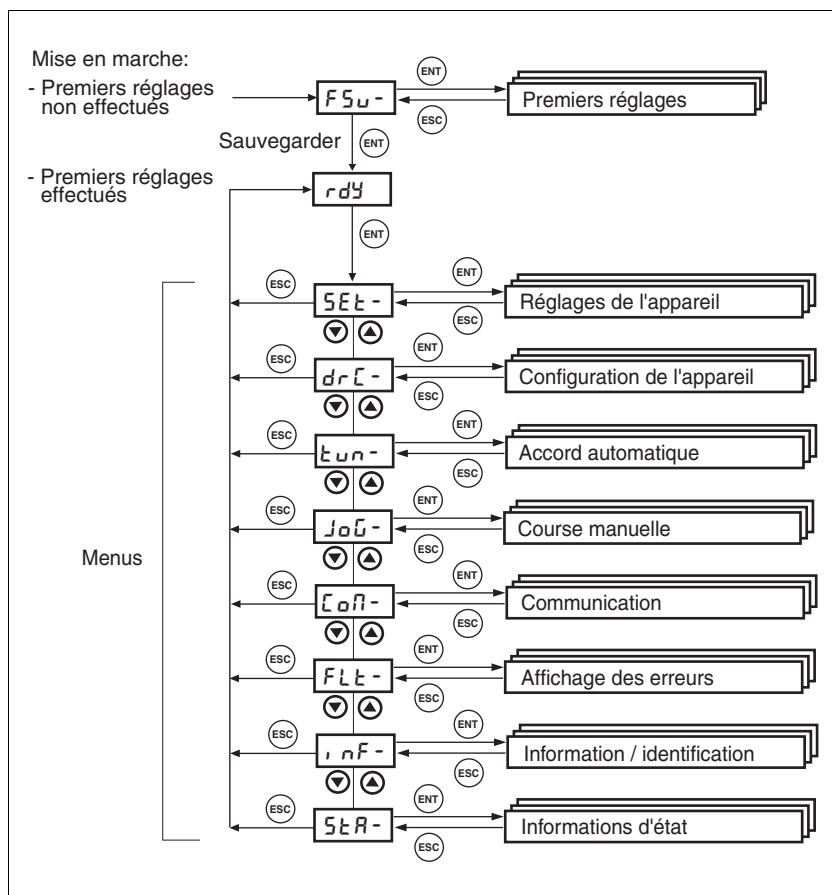
Illustration 7.5 Structure de menus HMI
